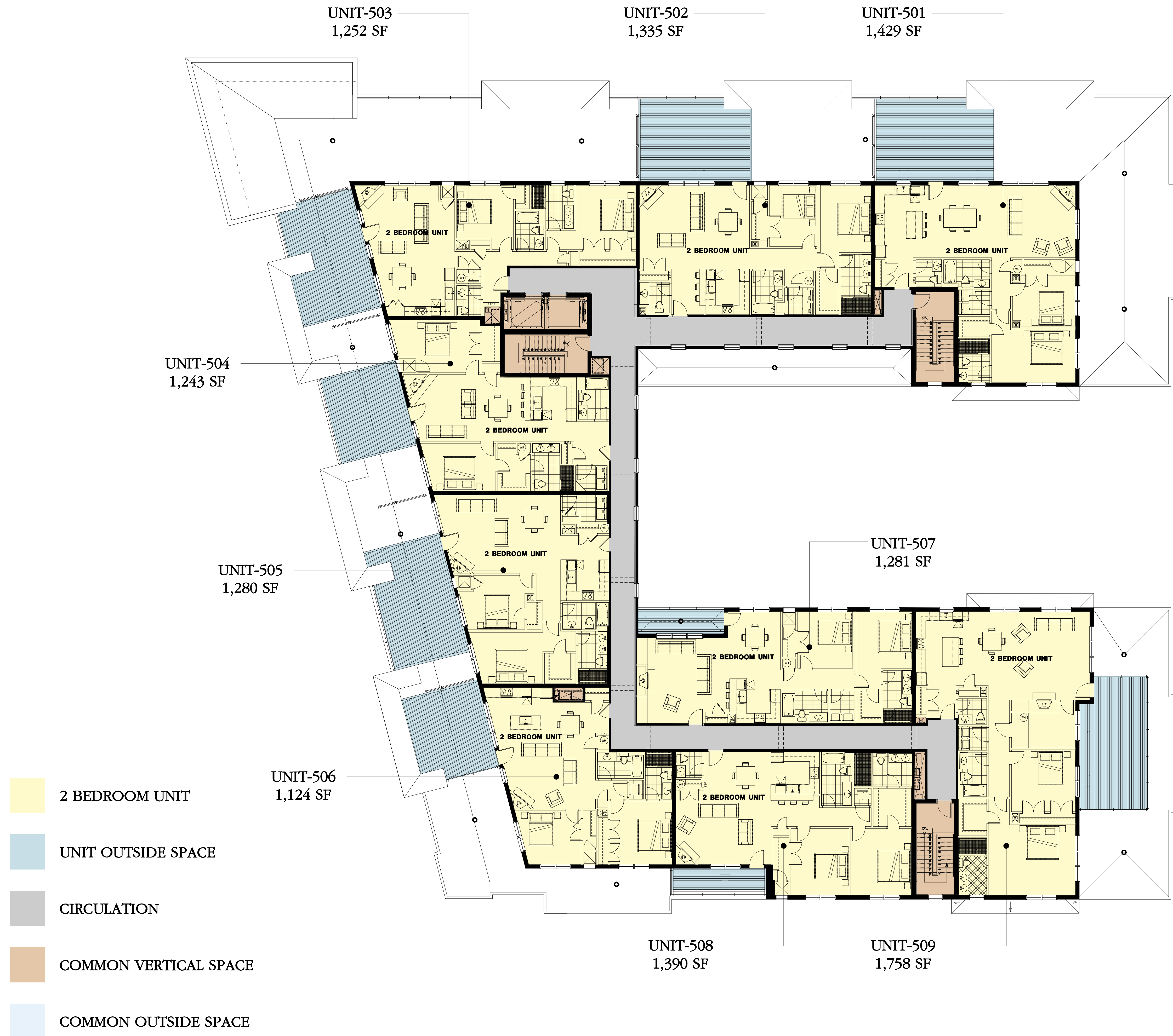
FIFTH FLOOR PLAN
